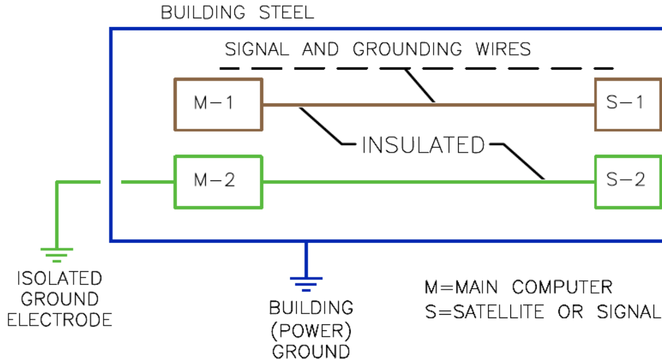
Figure 5-4—Isolated grounding of computers
